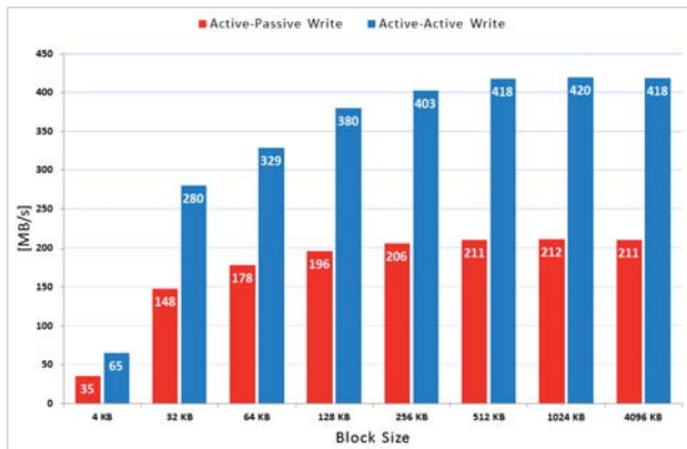
Figure 1. Write performance [MB/s] per block size (KB).
