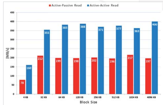
Figure 2. Read performance [MB/s] per block size (KB).
