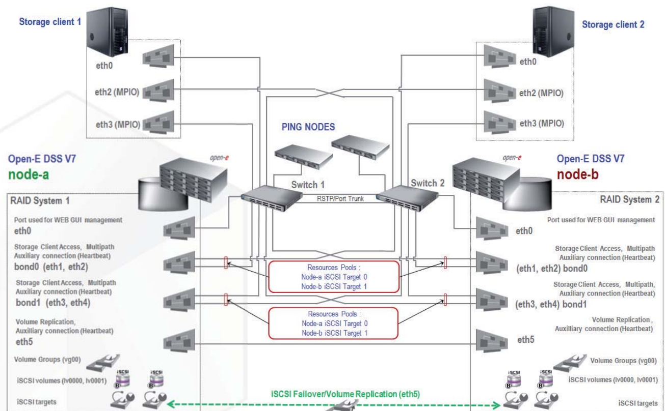
Figure 4. Hardware topology in test
