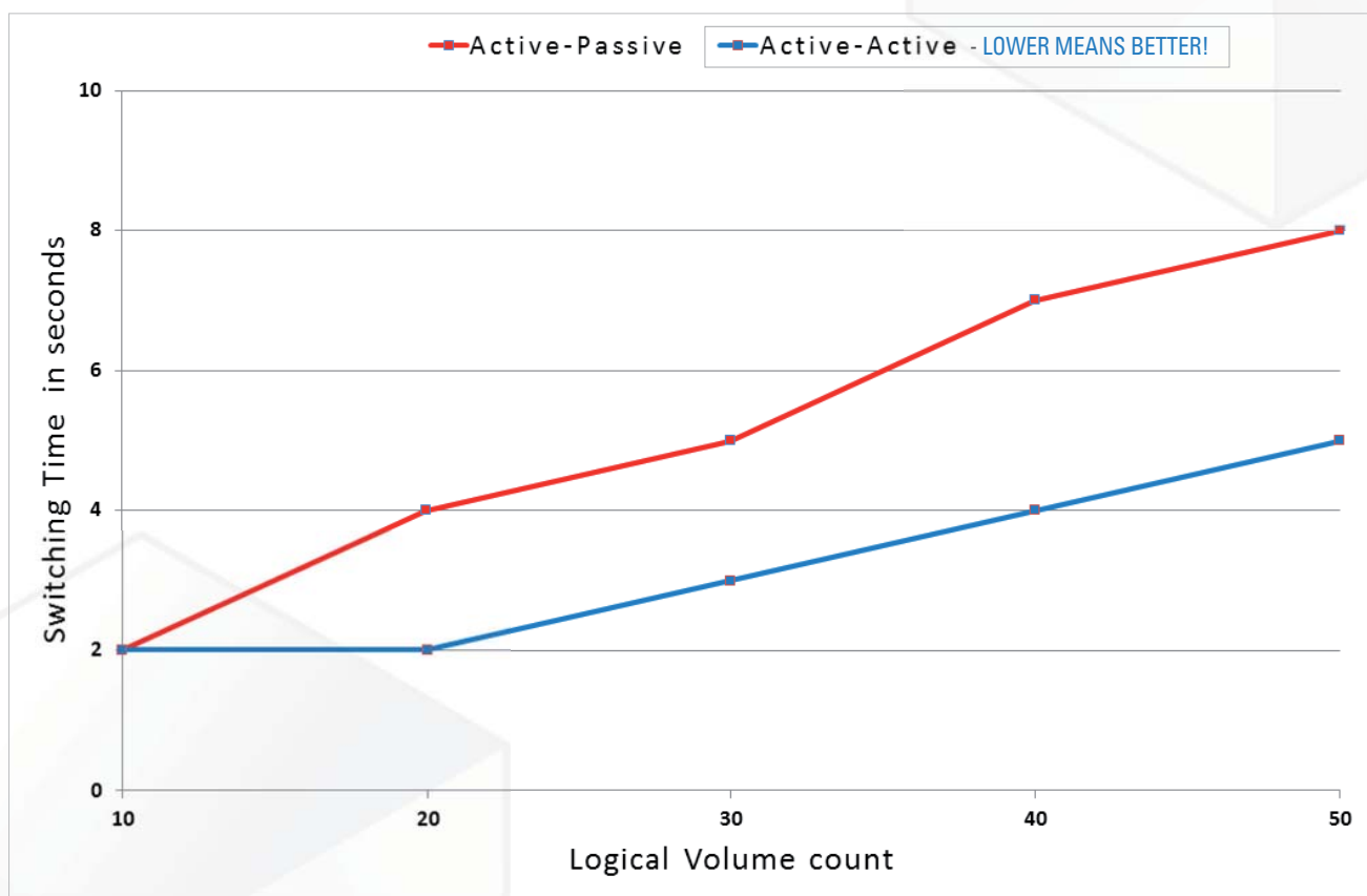
Figure 3. Failover switching time in seconds per LV count.
